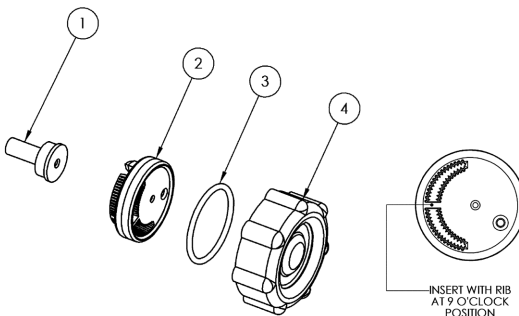
Figure 12: Injector Assembly
