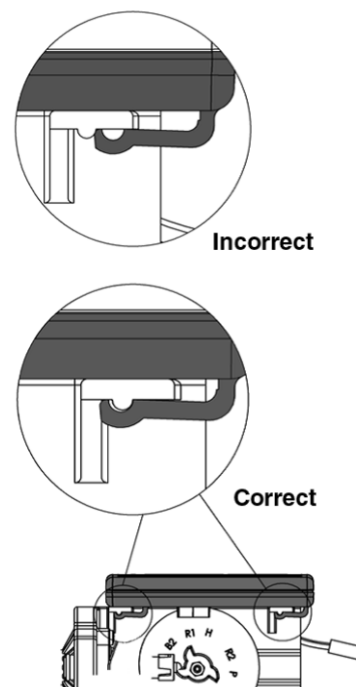
Figure 8: Controller Tab Lock Detail
