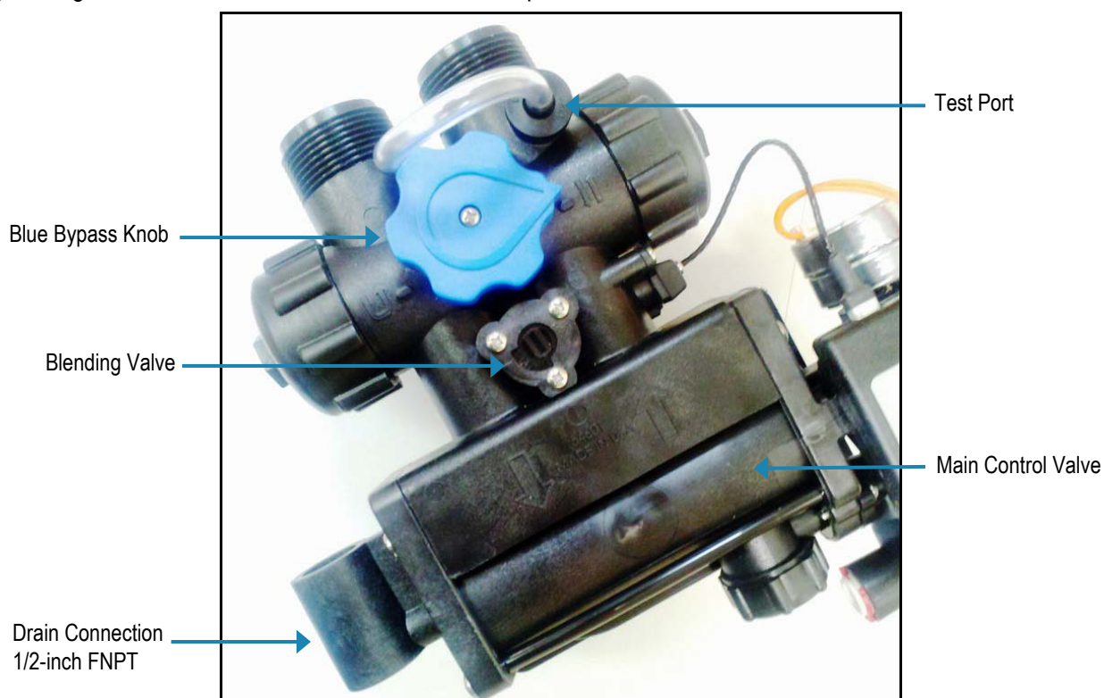
Figure 3: Bypass Valve
